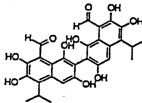
GOSSYPOL
